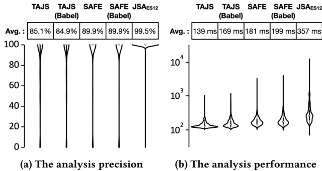
Figure 9: The analysis precision and performance for 3,878 tests soundly analyzable by all of five analyzers
