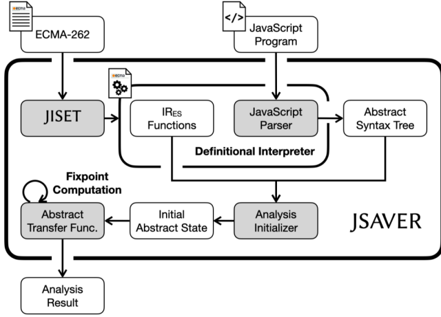
Figure 5: Overall structure of JSAYER
